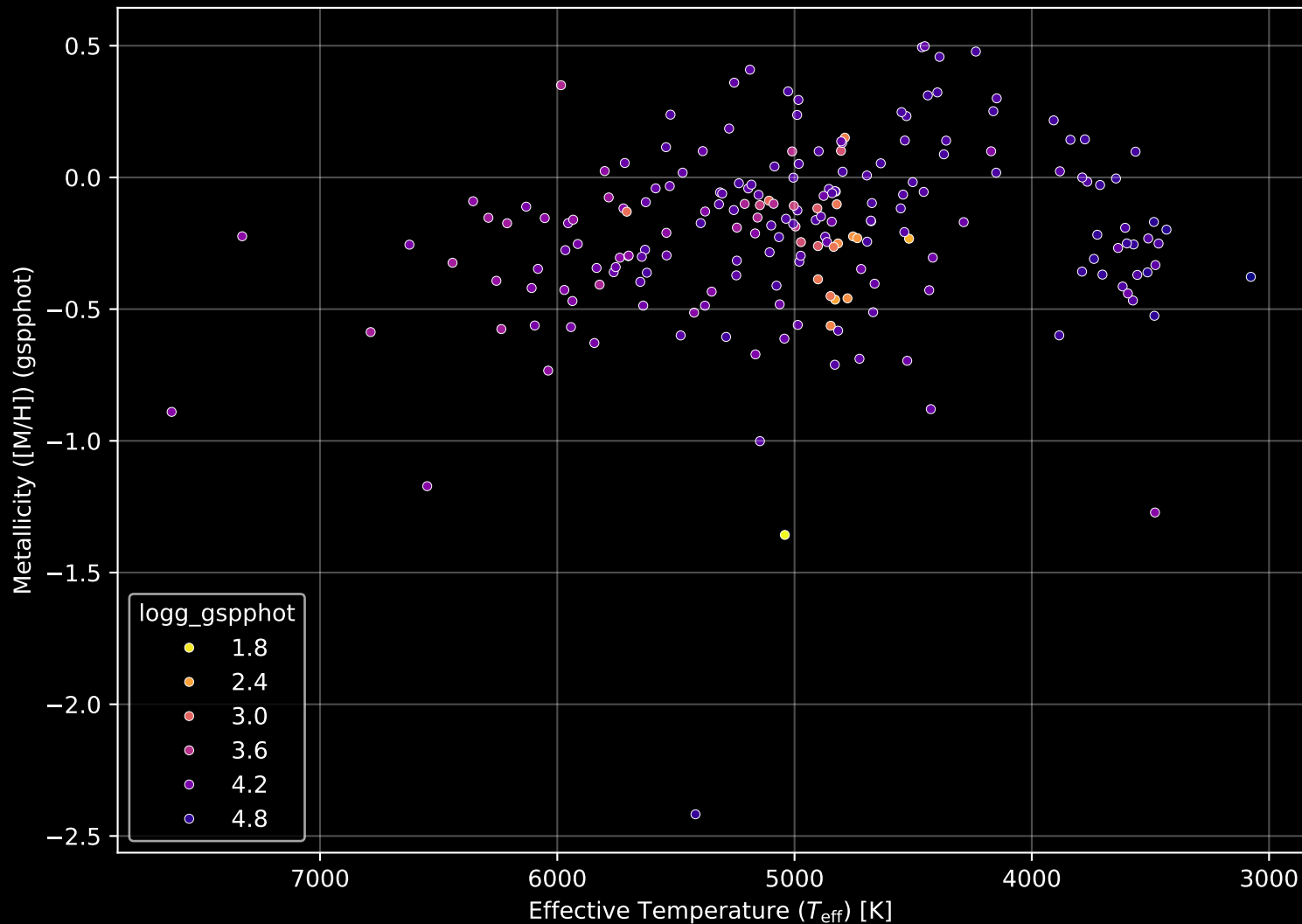
APOGEE DR17 Field: [K2_C8_125-59_btx] Stellar Population Parameters (n= 202)
