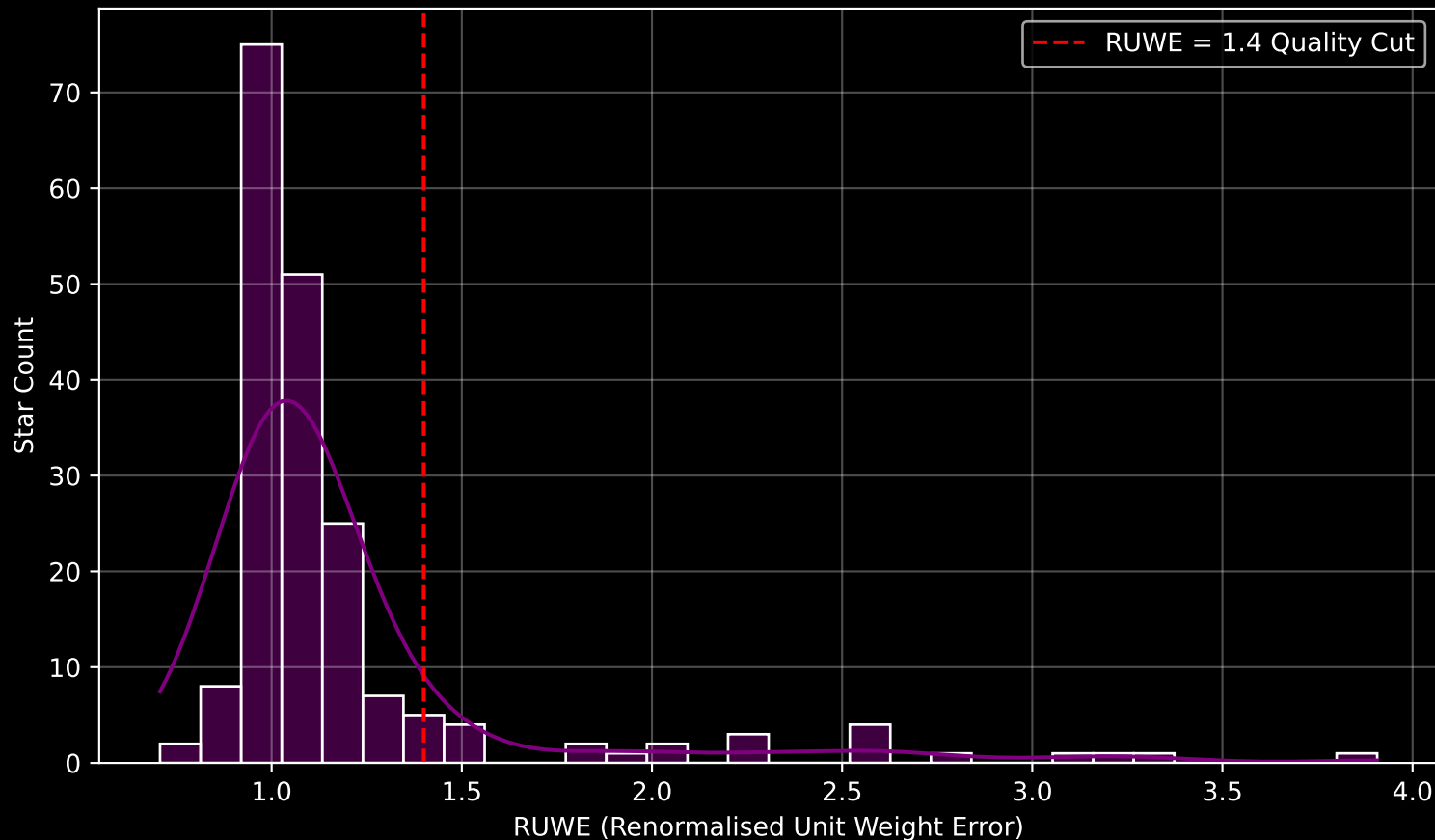
GAPOGEE DR17 Field [K2_C8_125-59_btx] RUWE Distribution (n= 194)
