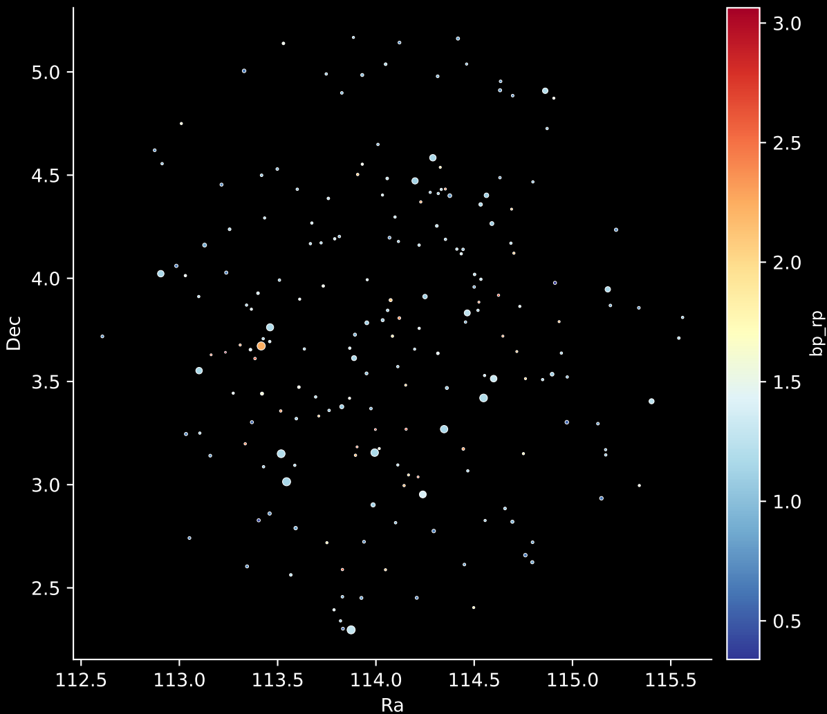
APOGEE DR17 Field: [K2_C8_125-59_btx] Stars: 202
