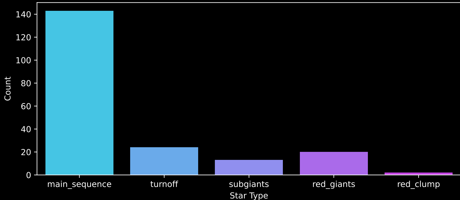
APOGEE DR17 Field: [K2_C8_125-59_btx] Count plot of Star Type
