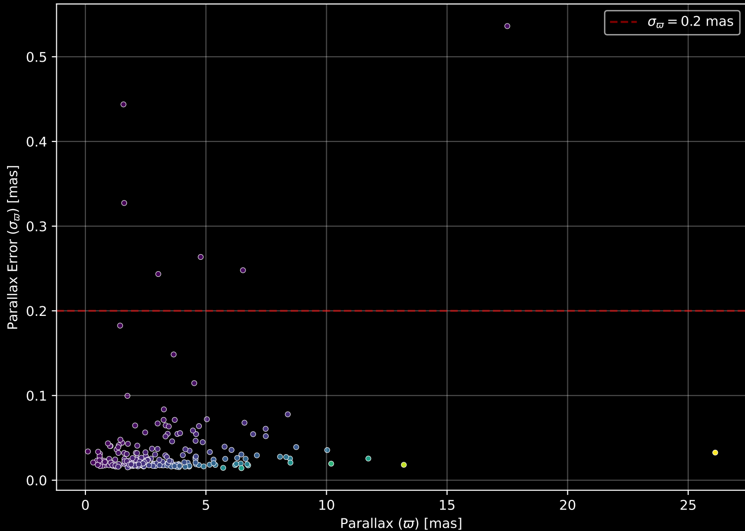
APOGEE DR17 Field: [K2_C8_125-59_btx] Parallax Quality (n= 202)
