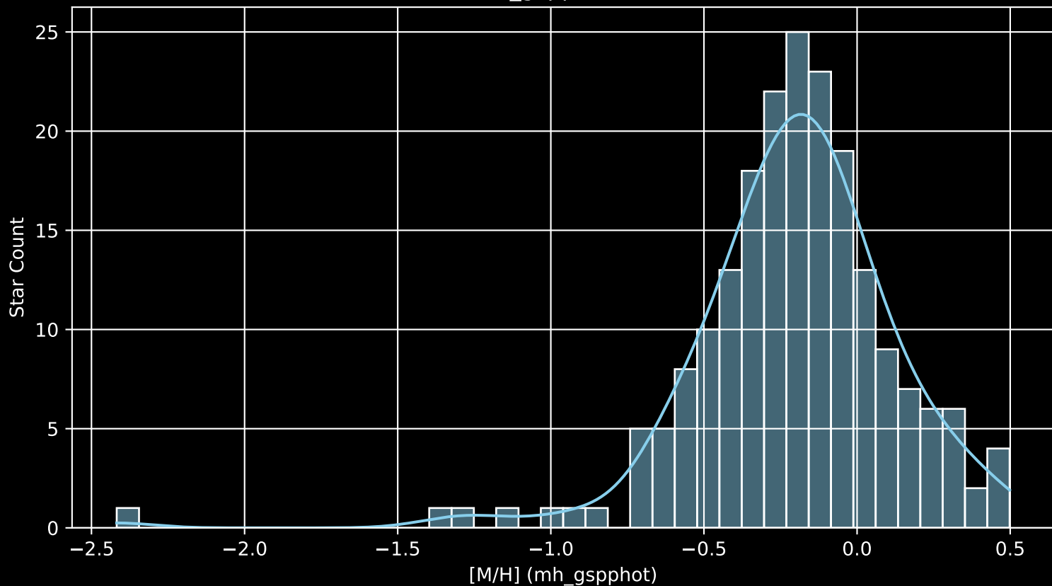
APOGEE DR17 Field: [K2_C8_125-59_btx [M/H] (mh_gspphot) (n= 202)
