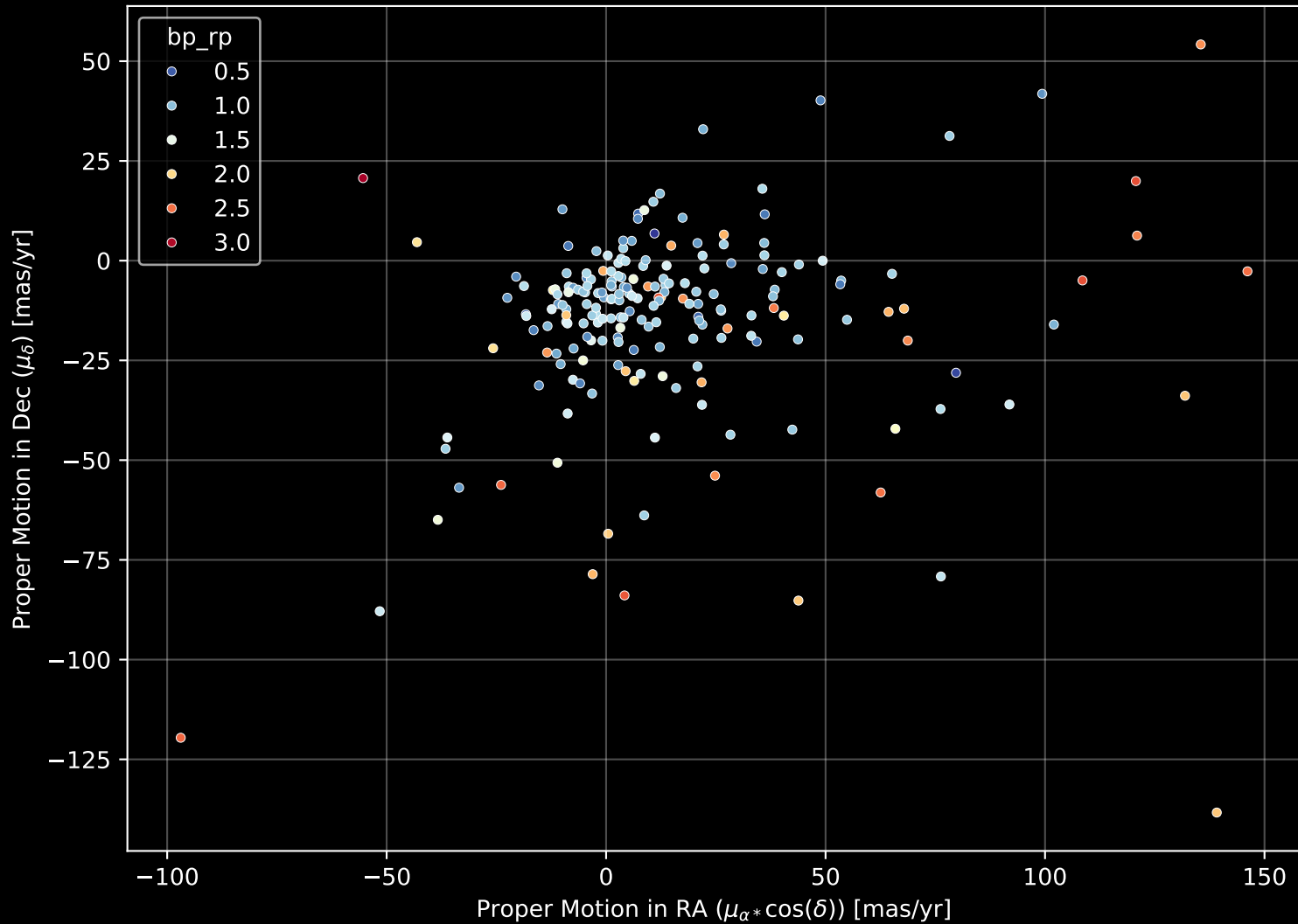
APOGEE DR17 Field: [K2_C8_125-59_btx] Proper Motion Diagram (n= 202)
